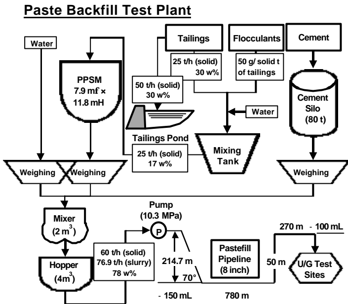
Figure 4 The flow sheet of the paste backfill plant constructed at the mill of the Toyoha Mine and transportation system to the underground test site (left) and the PPSM thickener (right).
