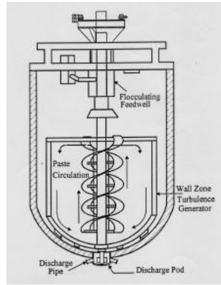
The PPSM thickener and its inner structure.
