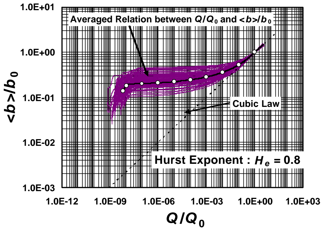
Figure 3 The relation between the normalized open apertures and volumetric flow rates obtained by the flow simulation using a set of 100 fracture models with the 2^6 \times 2^6 subdivisions and H_e = 0.8 .
