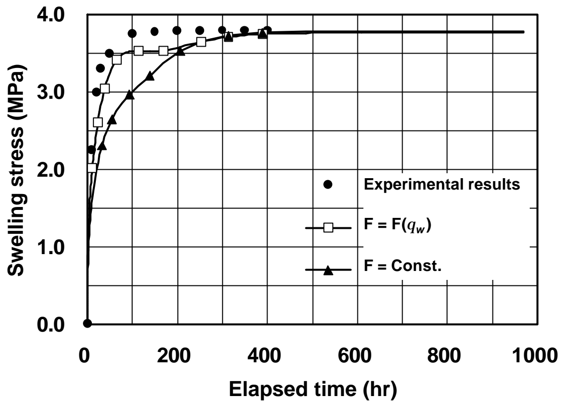
Figure 2 Comparison of swelling stress – time curves between experimental results and proposed models.
