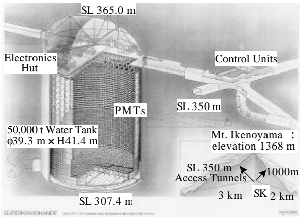
Figure 1 A schematic view of the Super-KAMIOKANDE.
